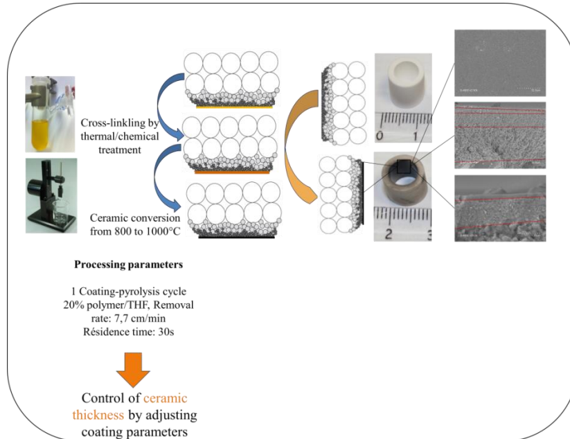
Figure 2: Experimental protocol for PDMCs elaboration.
