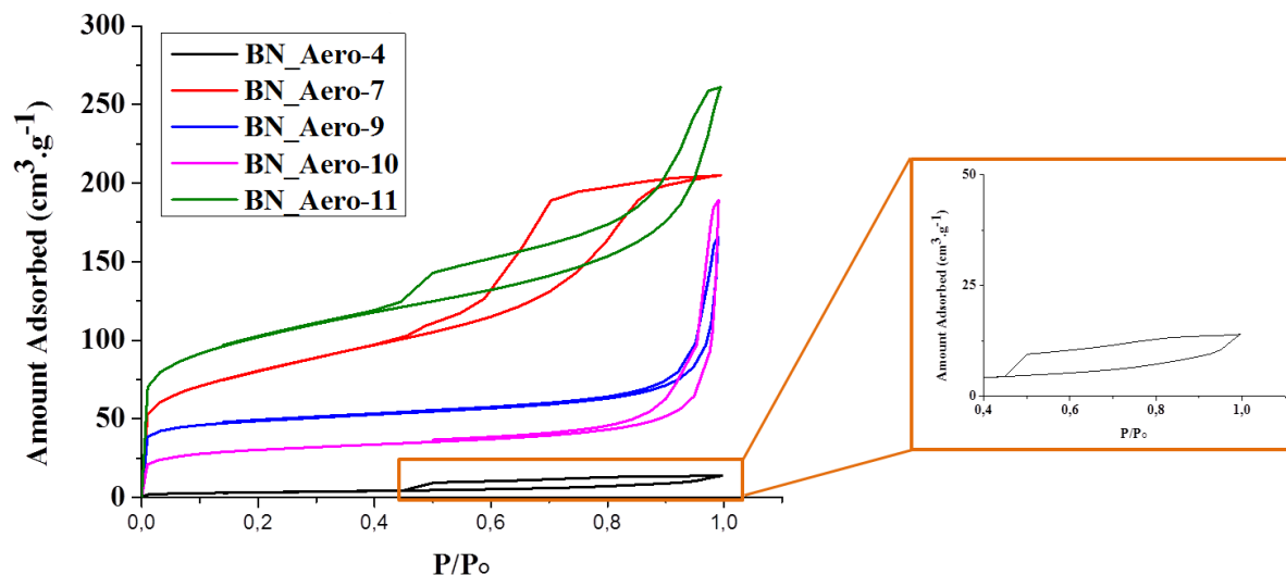
Figure III-16: N 2 adsorption-desorption isotherms of the BN aerogels .
