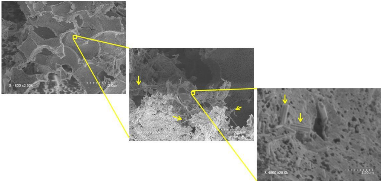
Figure V-31: SEM images of the HTTGA residue (PAAZ30/PMMA70-80-74-1800°C).
