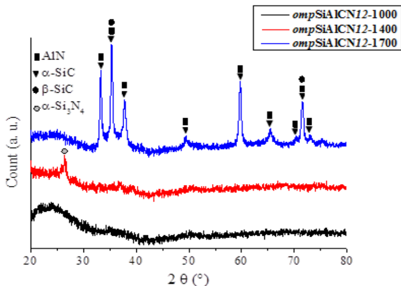
Figure IV-14: XRD patterns of ompSiAlCN12 at different temperatures.
