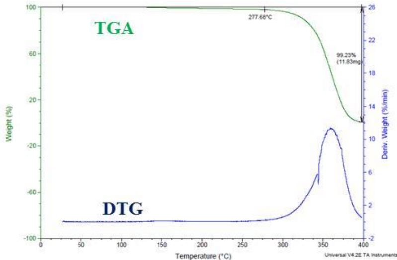
Figure V-25: TGA and DTG curves for PMMA-25 \mu\text{m} under \text{N}_2 with 5^\circ\text{C}\cdot\text{min}^{-1} as heating rate.
