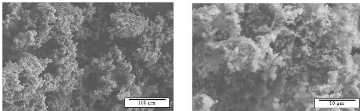
Figure IV-19: SEM images of ompSiAlCN12 after heat-treatment in air at 1000°C for 5 h.
