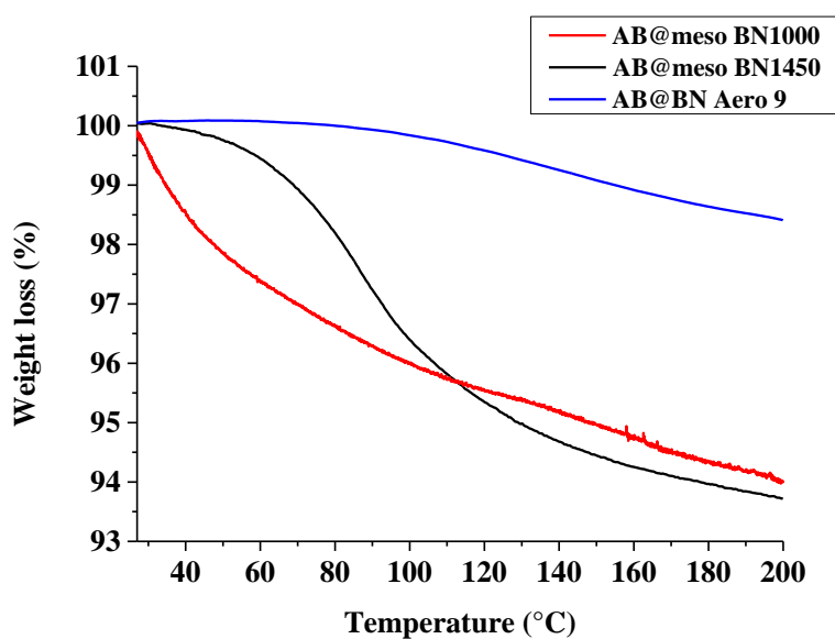
Figure ANNEX B-2: TGA curves of AB@mesoBN1000, AB@mesoBN1450 and AB@BN Aero 9 under \text{N}_2 up to 200 ^{\circ}\text{C} with a heating rate of 5^{\circ}\text{C}\cdot\text{min}^{-1} .
