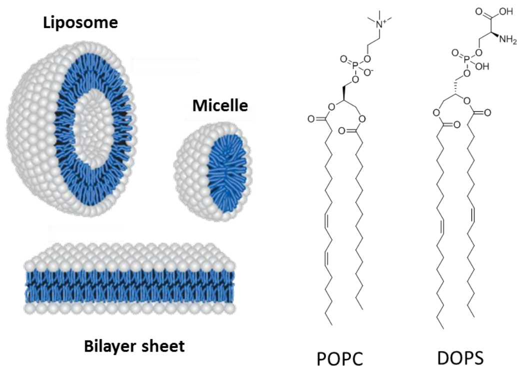
Figure 21. Lipid structures and most often used lipids
