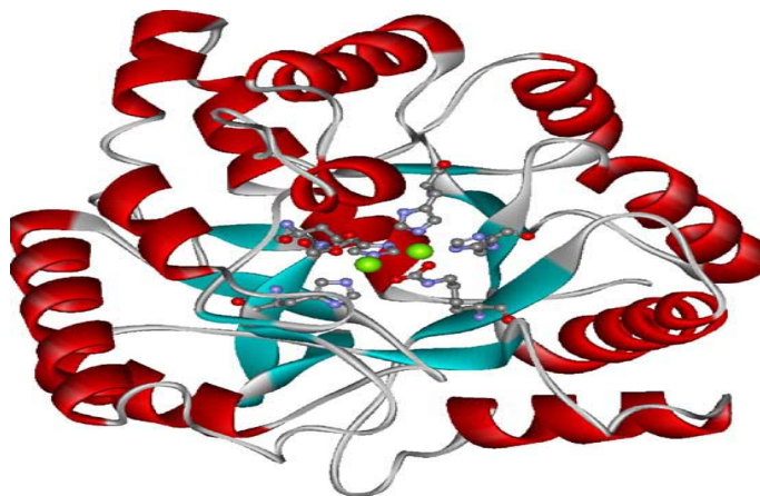
Fig. 4: Crystal structure of phosphotriesterase featuring a TIM barrel fold. Coordinates taken from PDB file 1 HZY [30].
