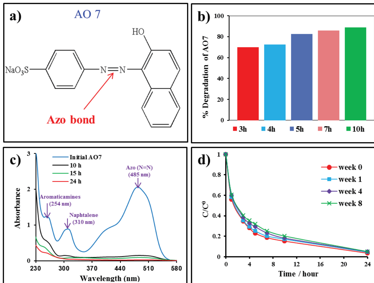
Figure 6-6. AO7 degradation by FC-Fenton system. (a) Molecular structure of AO7; (b) % removal of AO7 concentration as a function of treatment time; (c) Evolution of UV-Vis spectra of AO7 with treatment time. d) Degradation kinetics of AO7 recorded on 24 h from a fresh solution at week 0, week 1, week 4 and week 8. Conditions: 90 mL AO7 (0.1 mM) aqueous solution in 50 mM \text{Na}_2\text{SO}_4 with 0.20 mM \text{Fe}^{2+} at pH 3.0.
