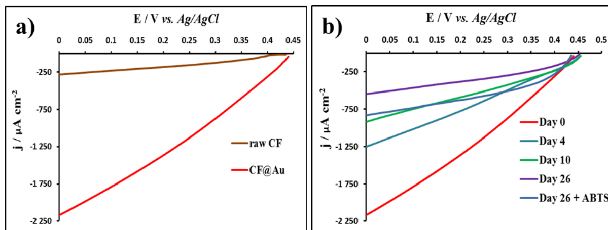
Figure 5-4. Enzymatic \text{O}_2 reduction on. (a) Polarization curves of \text{O}_2 electroreduction on the CF@Au and the raw CF biocathodes modified with the enzyme BOD. (b) Stability of the BOD-immobilized CF@Au electrode with time. Scan rate of 3 \text{ mV s}^{-1} , \text{O}_2 -saturated PBS 0.1 M, pH 7.0 at 30 \text{ }^\circ\text{C} .
