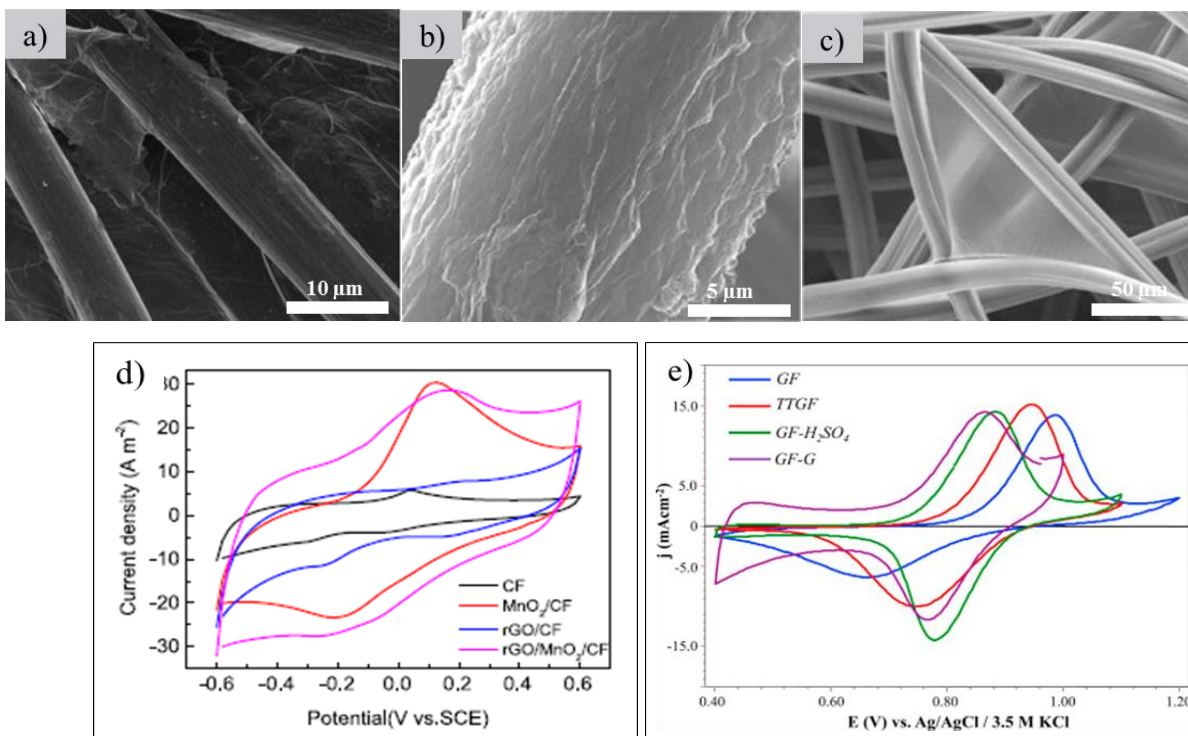
Figure 2-10. Characterization of graphene based felts. SEM images of rGO coated on (a) CF ( Shanghai Qijie Carbon Co., Ltd. ); (b,c) GF ( RVG-2000, Carbon-Lorraine company ); (d) CVs curves of the CF in 0.5 M \text{Na}_2\text{SO}_4 solution at a scan rate of 10 \text{mV s}^{-1} and (e) CVs recorded in a 0.05 M \text{VOSO}_4/1.0 M \text{H}_2\text{SO}_4 solution at a scan rate of 1 \text{mV s}^{-1} on the different GF electrodes [70, 75].
