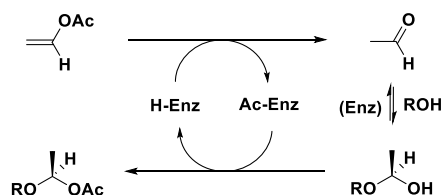
Scheme 3: Lipase-mediated HAE synthesis. 21,22
