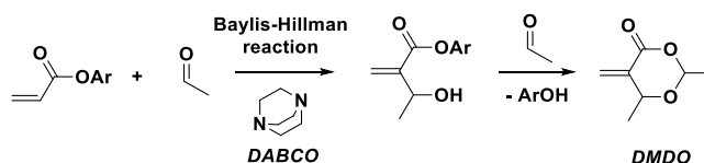
Scheme 18: DMDO synthesis by a Baylis-Hillman/cyclization sequence. 72
