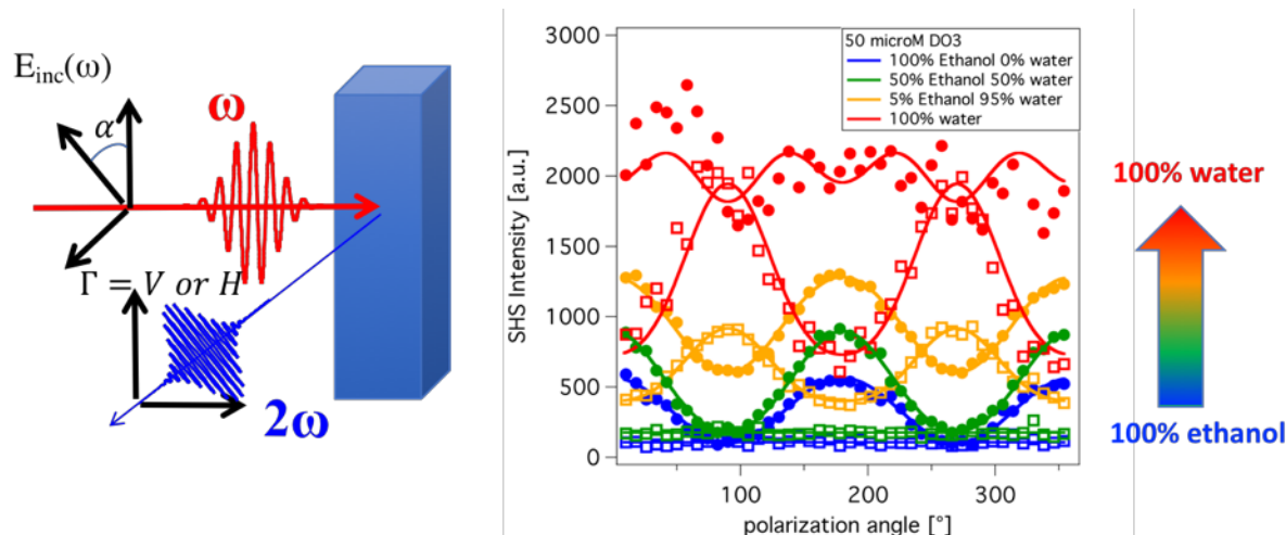
Figure 1. Left, the polarization resolved SHS experimental setup. Right, the SHS polarization plots obtained with [\text{DO3}] = 0.05 \text{ mM} for different ethanol-water ratio. The filled circle are I(\alpha, V_{\text{out}}) polar plot and empty square are I(\alpha, H_{\text{out}}) polar plot. The solid lines are a fit using the equation (2).
