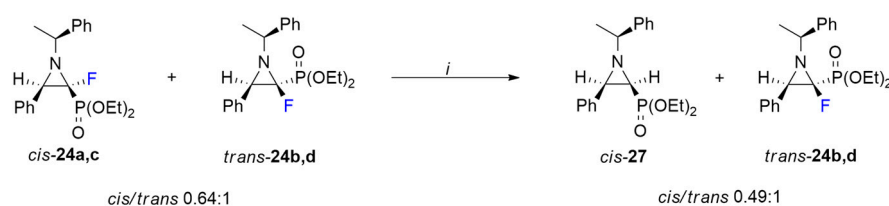
Scheme 5. Aziridine transformation with \text{NaBH}_4 . Reaction conditions: i . 24a–d (0.3 mmol), \text{NaBH}_4 (0.6 mmol), Pd/C (10 mol%), MeOH, 70 °C, 3 h. Note: For simplicity, only the stereochemistry of the major diastereomers was shown.
