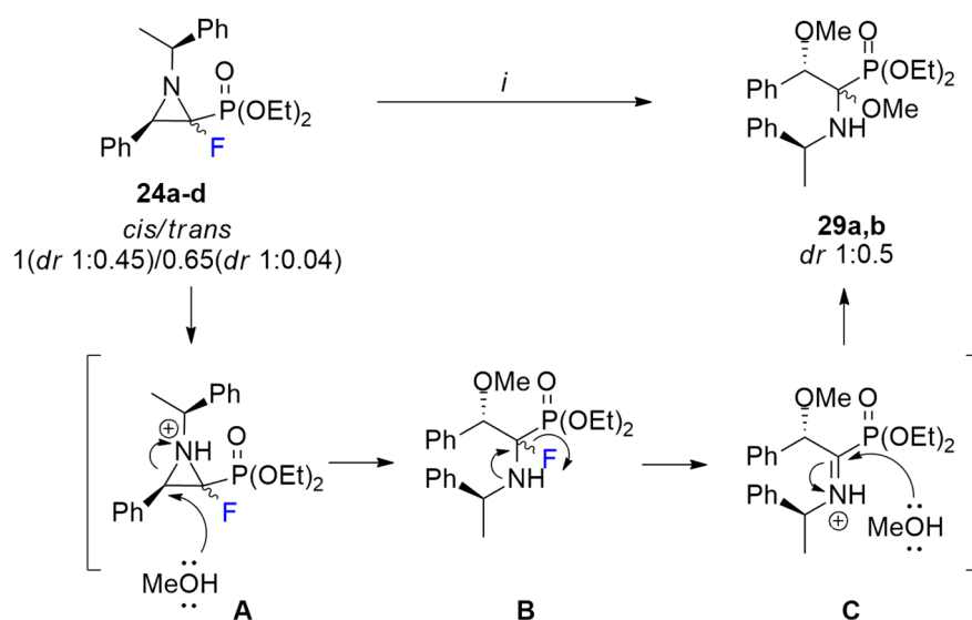
Scheme 6. Acid-catalyzed ring-opening reaction of 24a–d through intermediates A–C. Reaction conditions: i . 24a–d (0.5 mmol), \text{H}_2\text{SO}_4 98% (~0.5 mmol) MeOH, 70 °C, 2 h. Note: For simplicity, only the stereochemistry of the major diastereomers was shown.
