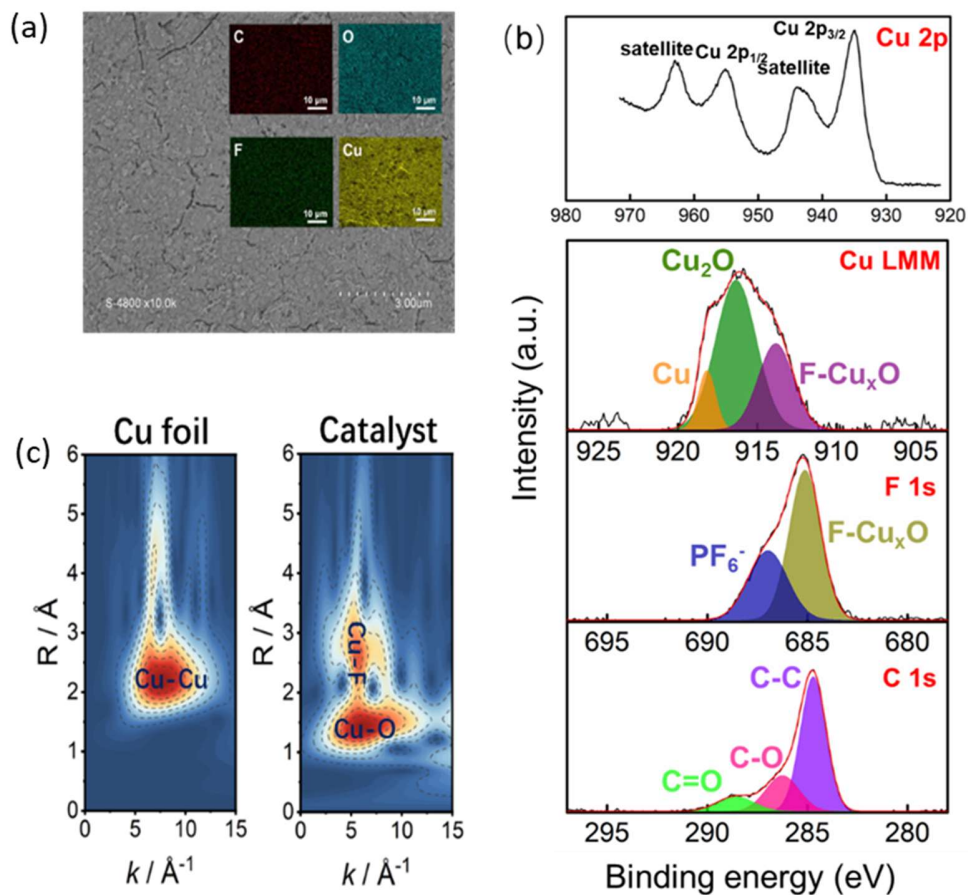
Figure 4. (a) SEM images (with the corresponding EDS mapping in the insets), (b) XPS spectra and (c) EXAFS wavelet transform 2D plot of the photochemical reaction product LiF-Cu 1.22 O@C (exposed 35 days to air) after the catalysis experiment. EXAFS results are compared to data obtained with the pristine Cu foil (on the left side).
