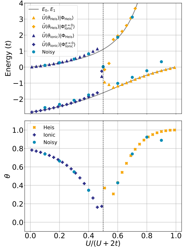
Figure 5: Energies of the half-filled Hubbard dimer for \Delta\mu/t = 2 (top panel) with respect to the repulsion strength, using the variational SW method to minimize the energies \langle\Phi_{\text{Heis}}|\hat{H}(\theta)|\Phi_{\text{Heis}}\rangle (orange markers, shown for U > \Delta\mu ) and \langle\Phi_{\text{Ionic}}^{\alpha=0}|\hat{H}(\theta)|\Phi_{\text{Ionic}}^{\alpha=0}\rangle (blue markers, shown for U < \Delta\mu ). The associated minimizing parameters \theta_{\text{Heis}} and \theta_{\text{Ionic}} are shown on the bottom panel, respectively. The vertical dotted line corresponds to U = \Delta\mu .
