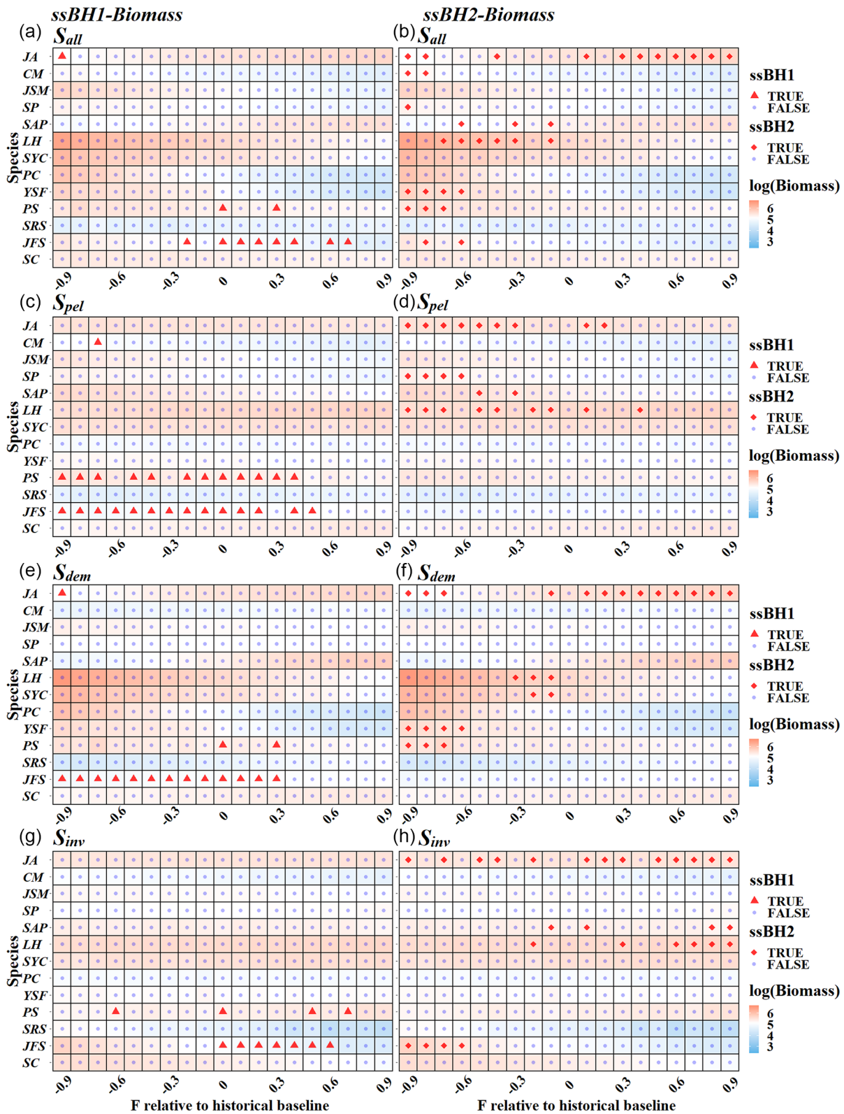
Figure 6. Change of biomass (in log scale) of each modelled species for four types of scenarios ( S_{all} : fishing for all species; S_{pel} : fishing for pelagic species; S_{dem} : fishing for demersal species; and S_{inv} : fishing for invertebrate). The fill colour from blue to red represents the log biomass from low to high. The red triangle indicates that ssBH1 occurs and the red diamond indicates that ssBH2 occurs, while the blue dot indicates that ssBH1 or ssBH2 does not occur.
