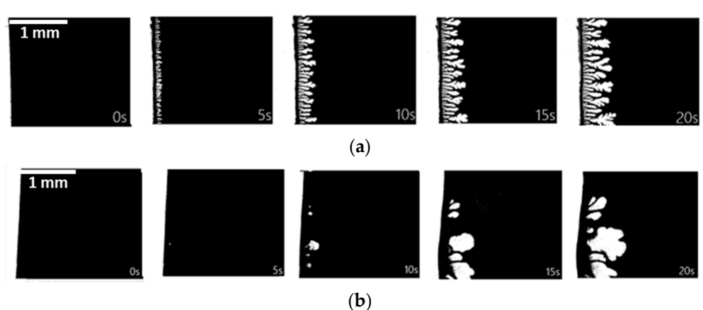
Figure 4. Binarized image series of water entrance to PVDF- \text{TiO}_2 solution at (a) 25 °C and (b) 70 °C.
