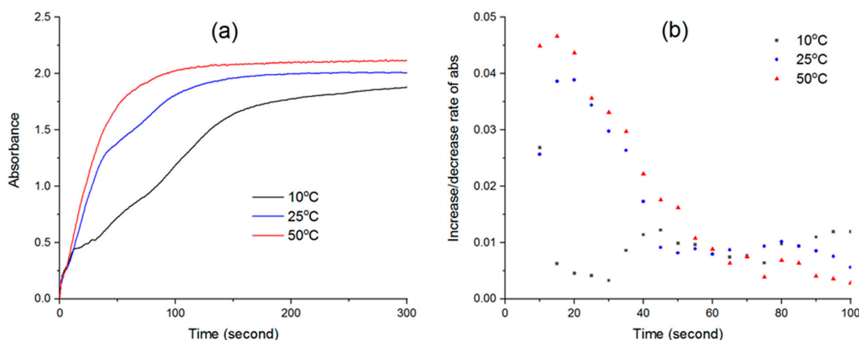
Figure 3. (a) UV absorbance over time of PVDF films immersed in water and (b) its increase rate.
