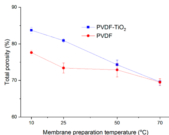
Figure 7. Membrane porosity.
