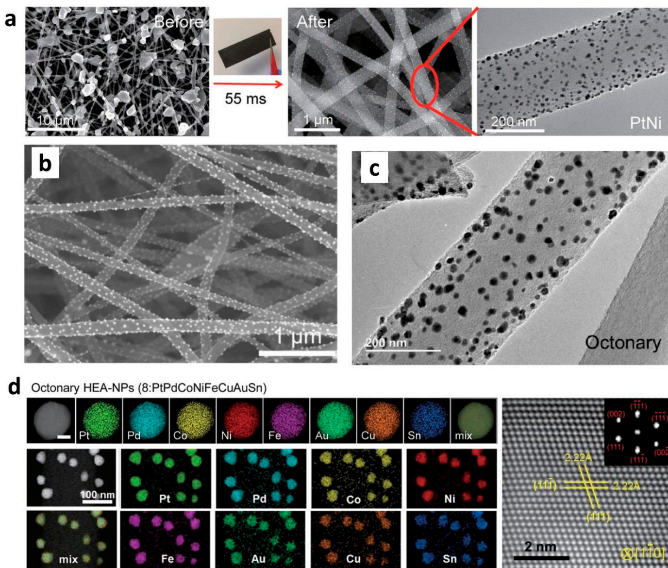
Figure 2. Nanoparticles loading onto carbon nanofibers derived from electrospun PAN nanofibers. (a) Illustration of carbothermal shock (CTS) method after electrospinning to synthesize high-entropy-alloy nanoparticles (HEA-NPs): SEM images of microsized precursor salt particles before and after CTS. (b–d) SEM, TEM, and HAADF-STEM mapping images of octonary alloy nanoparticles. Reprinted and adapted with permission from ref. [65]; Copyright 2018, AAAS.
