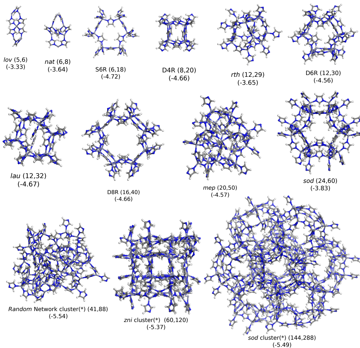
Figure 7: Geometries and energies (in eV, in parenthesis) of some relevant large clusters, with a number of Zn^{2+} cations ranging from 5 to 144. The number of Zn^{2+} cations and Im^- ligands are shown using the (z, l) notation. The energy is calculated from the linear regression reported in Figure 6. Color code as in Figure 1.
