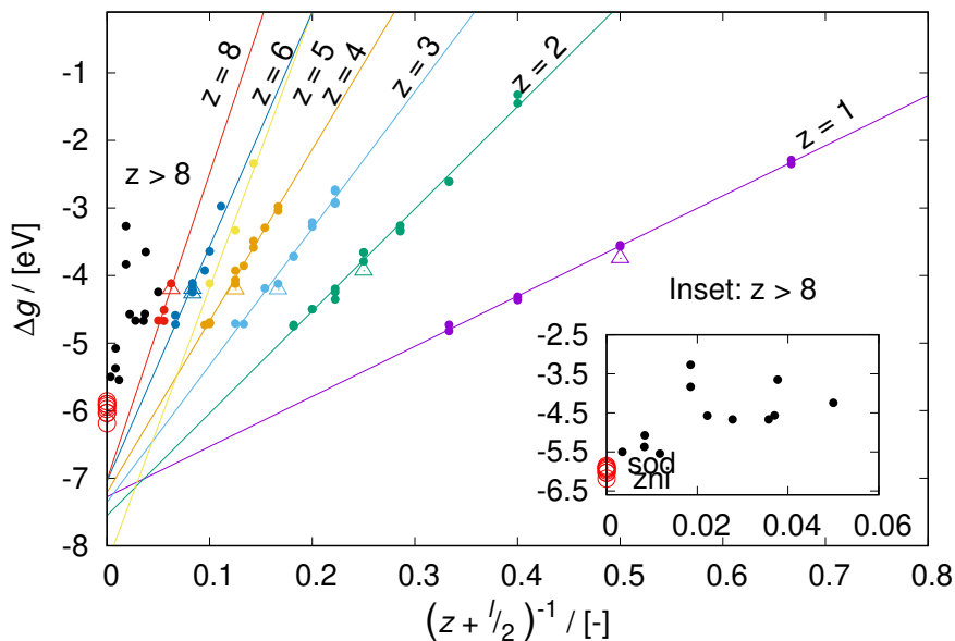
Figure 8: Values of formation free energy per Zn atom, \Delta g , of \text{Zn}_z\text{L}_l clusters ( l = lm^- and mlm^- ) as a function of the number of Zn atoms and the number of ligands, (z + 1/2)^{-1} , calculated with three types of calculations, namely the periodic meta-GGA exchange-correlation functional SCAN+rVV10, with the GFN2-xTB method, and with the non-periodic, hybrid exchange-correlation functional \omega\text{B97X}/6\text{-311++G(d,p)} . Each line represents a fitting of the cluster energies corresponding to a particular value of z (with different number of ligands, l ). The black circles correspond to the energies of the clusters with z > 8 . Red empty circles correspond to the energies of the crystalline materials calculated with the GFN2-xTB method ( zni , cri , coi , ZIF-1, ZIF-4, ZIF-6, ZIF-8, SALEM-2, and ZIF-10). Empty triangles correspond to fitted \Delta g of the corresponding cluster calculated with the periodic meta-GGA exchange-correlation functional SCAN+rVV10. These values are obtained following the methods described in the ESI. The inset shows the region of larger clusters and of periodic systems.
