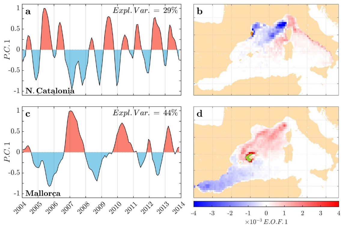
Figure 3. Prevailing sources and interannual patterns of LPDP arriving at the target areas after eight months. Temporal ( a,c ) and spatial ( b,d ) representation of the first principal component (PC1) of empirical orthogonal function (EOF) analysis conducted on source areas of individuals based on 120 monthly origin maps (2003–2014) (more details in “Methods”). The results are for N. Catalonia ( a,b ) and Mallorca ( c,d ). The total explained variance was 29% for N. Catalonia and 44% for Mallorca. Positive PC and EOF values are in red, and negative values are in blue. Original source maps can be reconstructed using the climatology (Fig. 1b,c) and adding the product of PC1 by EOF values. Therefore, intensified influence as source areas emerges when blue/red areas (from EOF value) and PC value match (blue/red). The figure and superimposed maps were created using “M Map: A mapping package for MATLAB”, v.1.4m ( www.eoas.ubc.ca/~rich/map.html ) in MATLAB v.R2010b ( www.mathworks.com ).
