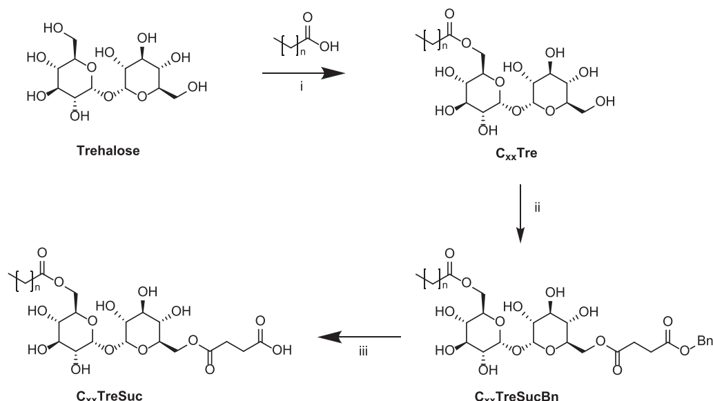
Fig. 1. Synthesis of Trehalose derived ionic surfactants. Reagents and conditions: i - Fatty acid ( n = 6, 8, 12, 14 ), TBTU, pyridine 96 hr. ii - SAMBE, TBTU pyridine 96 hr. iii - \text{H}_2 Pd/C, MeOH 3 hr.
