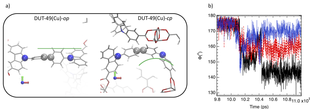
Fig. 4 (a) Illustration of the typical angular deflection in both DUT-49(Cu)-op and DUT-49(Cu)-cp. (b) Time evolution of three angular deflections, \phi_1 (black), \phi_1 (red) and \phi_3 (blue) randomly selected during the op \rightarrow cp transition.
