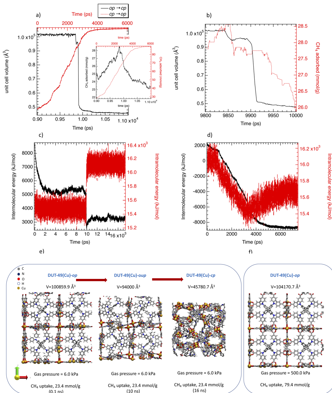
Fig. 3 (a) OMD simulated unit cell volume changes alongside the \text{CH}_4 -triggered op – cp and cp – op structural changes. Inset figure represents the corresponding \text{CH}_4 adsorbed amount with the same color code. (b) Enlargement of part a between 9.8 ns and 10 ns. Intermolecular and intramolecular energy as a function of time during the op \rightarrow cp (c) and cp \rightarrow op (d) transitions. (e) Illustrations of the DUT-49(Cu) structure configuration during the structural transitions: op , cp and unstable phases. (f) Illustration of the final configuration of DUT-49(Cu) for a \text{CH}_4 pressure of 500 kPa.
