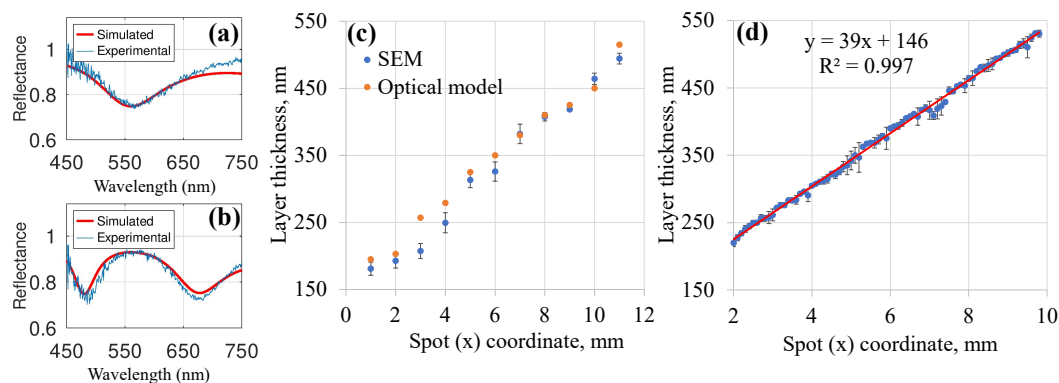
Figure 3. (a,b) Measured and calculated reflectance spectra at different layer thicknesses, 260 and 520 nm, of ZnO NR-PAAO hybrid film on Al substrate. (c) Comparison of hybrid film thickness measurements at different sample positions (x coordinate) obtained by SEM and fitting the reflectance spectra (optical model). (d) Hybrid film thickness profile obtained using reflectance measurements.
