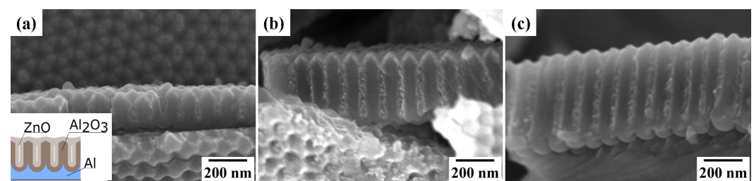
Figure 1. (a–c) Cross section SEM images of variable-thickness ZnO NR–PAAO hybrid film from the same sample at different positions (x coordinates). The inset shows a schematic of the sample morphology.
