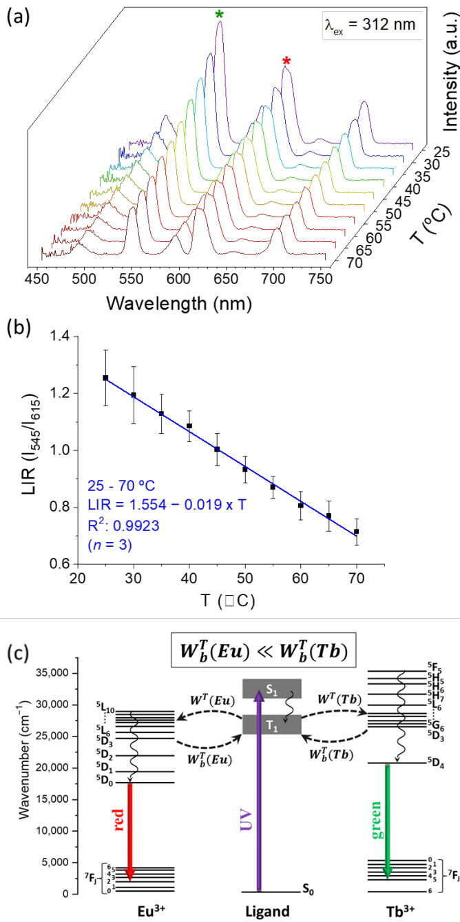
Figure 6. (a) Emission spectra of IONP@SiO 2 -acac-Ln 3+ ( \lambda_{\text{ex}} = 312 \text{ nm} ) recorded at temperatures between 25 and 70 °C. The green and red asterisk symbols indicate the \text{Tb}^{3+}: \ ^5\text{D}_4 \rightarrow \ ^7\text{F}_5 (530–565 nm) and \text{Eu}^{3+}: \ ^5\text{D}_0 \rightarrow \ ^7\text{F}_2 (603–637 nm) transitions, of which integrated areas were used to construct (b) the calibration curve LIR vs. temperature. The solid line represents a linear fitting. The error bars correspond to standard error of mean determined from three consecutive temperature cycles. (c) Simplified energy level diagram showing the intra-4f transitions observed in Figure 5b and the effect of the increase of the backward IET rates W_b^T with the temperature; see SI for further details on the IET calculations.
