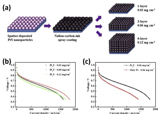
Figure 8. (a) Schematic representation of controlled sputter-deposited Pt 3 Y nanoparticles; (b) voltage-current curves of Pt 3 Y as function of deposited Pt layers; and (c) voltage-current curves comparison between optimized Pt 3 Y and Pt (Reproduced from Ref. [43] with permission from Elsevier. Copyright 2022).
