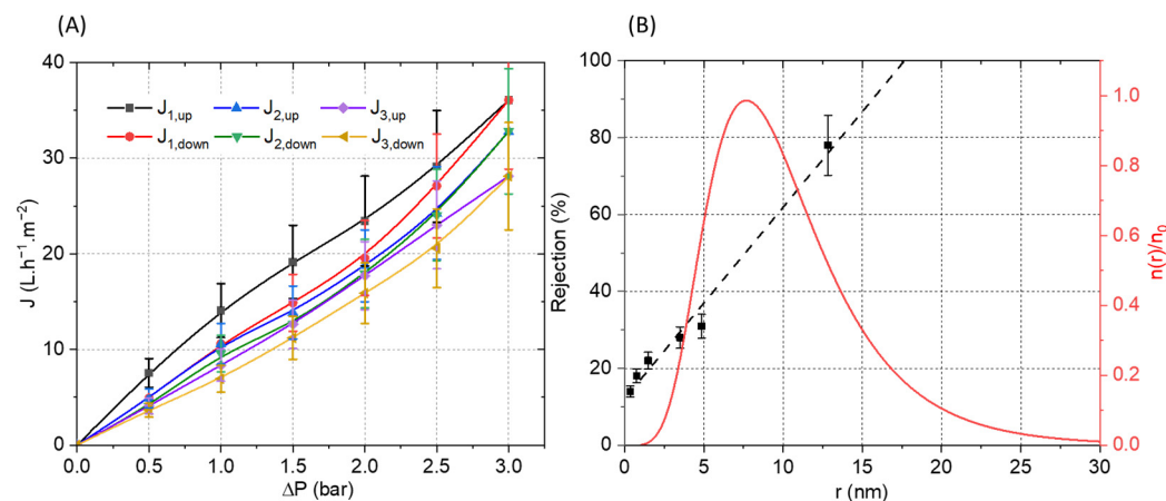
Figure 10. (A) Pressure increase and decrease cycles of water permeation experiment with the PVDF-supported membrane. (B) Polyethylene glycol (PEG) rejection coefficient ( R ) vs. the Einstein–Stokes radius of the solute (PEG) (black). Log-normal pore size distribution: reduced number of pores per unit of area n(r)/n_0 vs. the pore radius (red).
