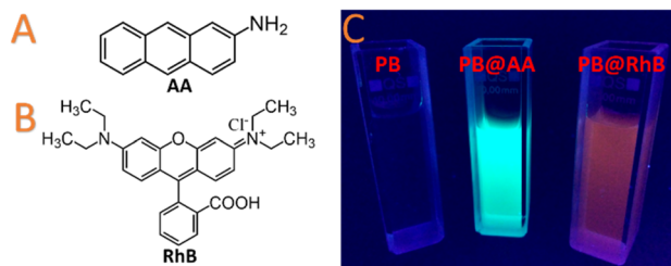
Fig. 8 (A) Scheme of the 2-aminoanthracene (AA); (B) scheme of the rhodamine B (RhB); (C) photographs of aqueous suspensions of PB, PB@AA, and PB@RhB under excitation with a UV lamp at 365 nm showing their luminescence. Reprinted with permission from ref. 167. Copyright 2020 American Chemical Society.
