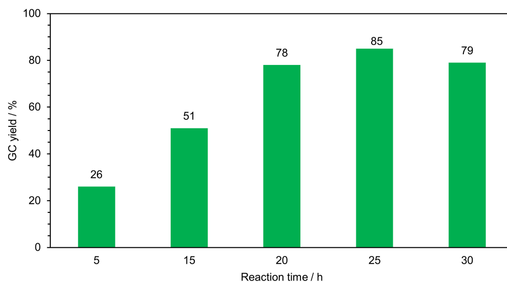
Figure 11. Effect of the reaction time on the product yield. Reaction conditions: 1,1-diphenylethylene (0.3 mmol); THF (1 mL); DTBP (4 equiv.); KI (20 mol%), \text{Cu}_1\text{Ce}_{0.7}\text{Si} catalyst (8.4 mg–4.8 mol%); 120 °C; under air.
