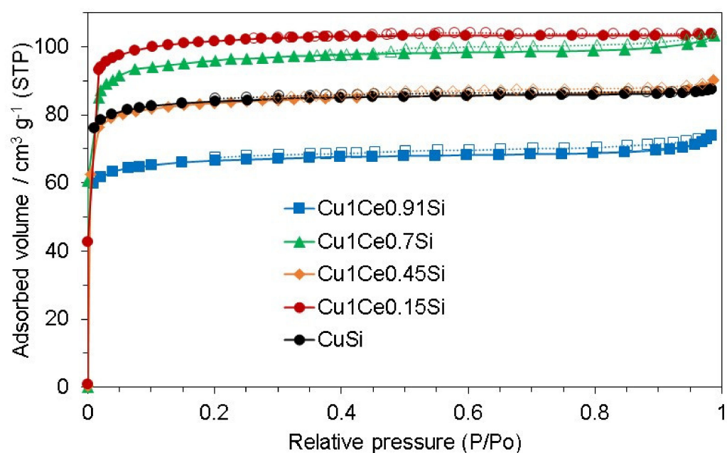
Figure 4. N 2 -physorption isotherms of the combustion-synthesized composites.
