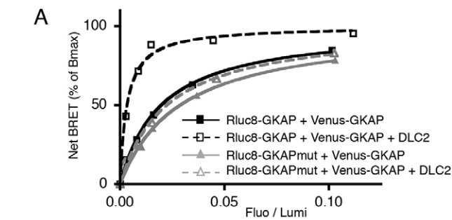
Fig. 2. GKAP forms dimers, which are favored by the interaction with DLC2. (A) HEK293 cells were co-transfected with constant concentrations of RLuc8-GKAP or Rluc8-GKAPmut and increasing concentrations of Venus-GKAP, with or without DLC2 expression plasmids. BRET was expressed as a function of the Venus-GKAP acceptor expression level. Individual readings obtained from three independent experiments were pooled. The curve was fitted using a nonlinear regression equation (GraphPadPrism), assuming a single binding site. (B) HEK293 cells transfected with the indicated expression plasmids were treated with NHS-LC-Diazirine (SDA), to cross-link the oligomers, or left untreated. The dimer:monomer ratio of Cerulean-GKAP and Cerulean-GKAPmut proteins were quantified by western blot analysis using the anti-GFP antibody. Actin staining was used to control protein loading. (C) Cells were transfected as in B, and all conditions were cross-linked with SDA. mCherry-DLC2 expression was assessed by using the anti-RFP antibody. The dimer:monomer ratio of Cerulean-GKAP in each condition was expressed as a percentage of the ratio obtained with Cerulean-GKAP alone. Data show the mean \pm s.e.m. (three individual experiments); *** P < 0.0001; NS, non-significant (Mann-Whitney U -test).
