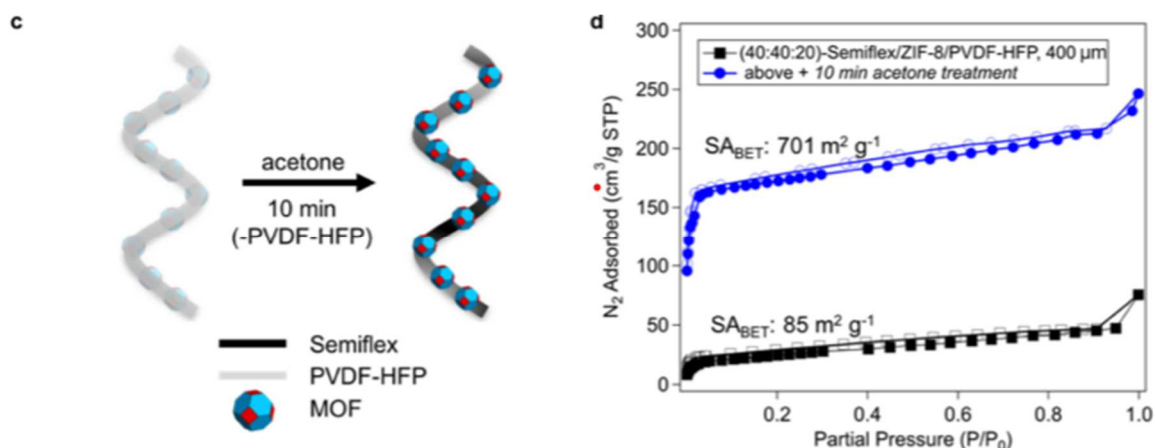
Figure 5 N 2 adsorption/desorption isotherms of Semiflex/ZIF-8/PVDF-HFP 400 \mu m strands as printed and after acetone treatment. Reprinted with permission from [15]. Copyright 2020 American Chemical Society.
