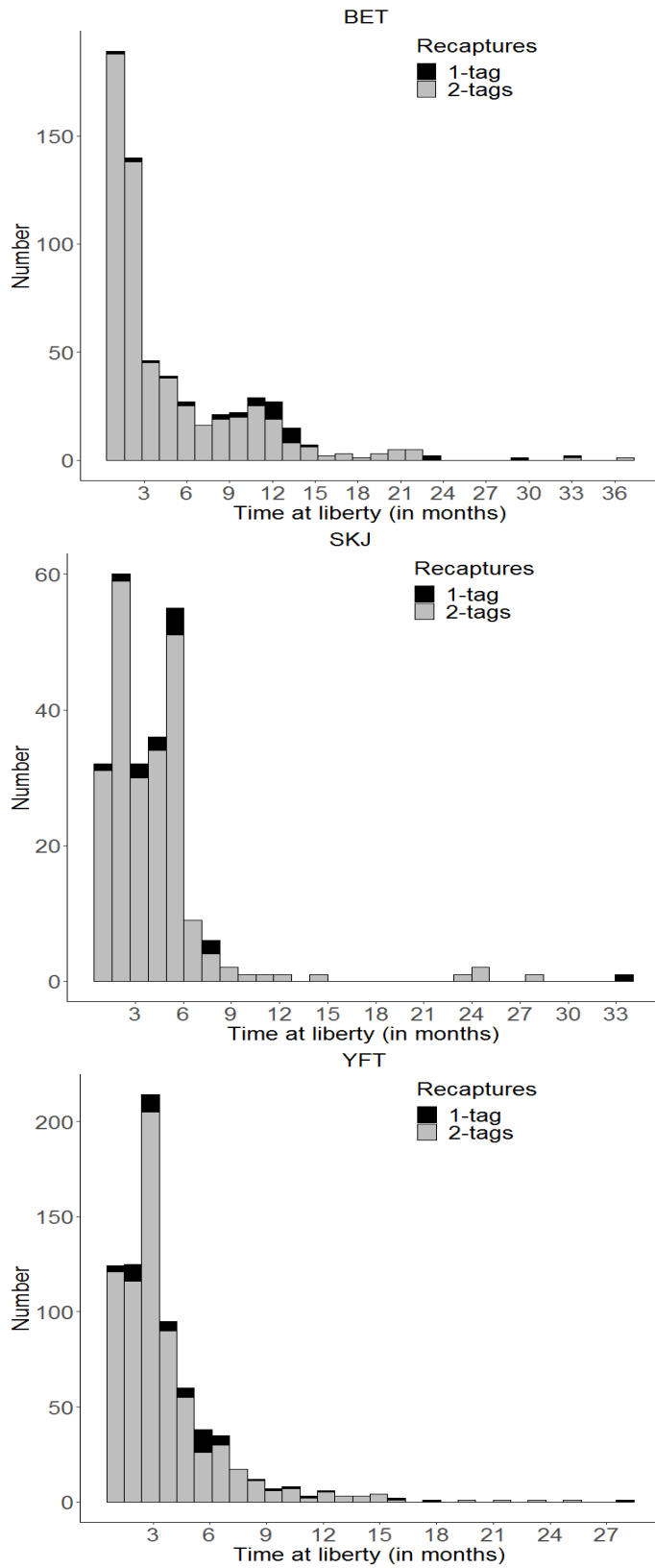
Fig. 2. Recaptures by time at liberty of tunas with 1 or 2 tags. From top to bottom: Bigeye (BET), Skipjack (SKJ), Yellowfin (YFT). Each bin represents one month at sea.
