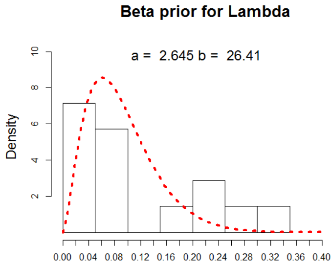
Fig. 1. Hyper-parameters of the Beta prior distribution (dashed line in red) for type I and II tag-shedding rates obtained from previous double-tagging experiments (histogram) conducted on different species of tunas in different parts of the world (see table 2).
