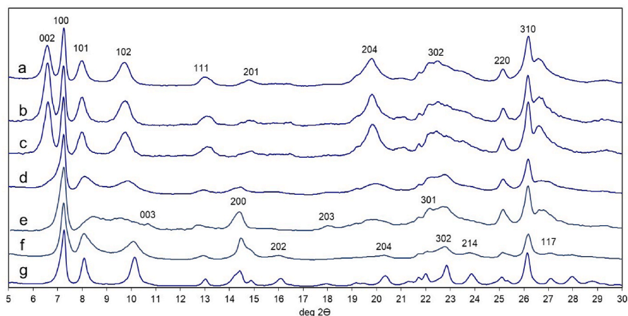
Fig. 3. Evolution of the XRD pattern of MWW(P) upon treatment by diluted HNO 3 in organic solvent and calcination: samples MWW(P) (a), pH4 (b), pH3 (c), pH2 (d), pH1 (e), pH1C (f), MWW(P)C (g).
