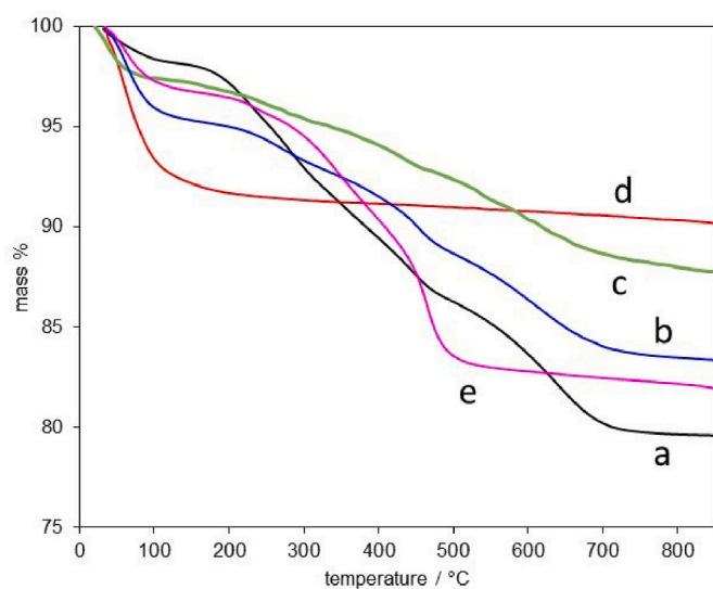
Fig. 7. TG curves of samples. MWW(P) (a), pH2 (b), AA (c), MWW(P)C (d), CupH4E-2 (e).
