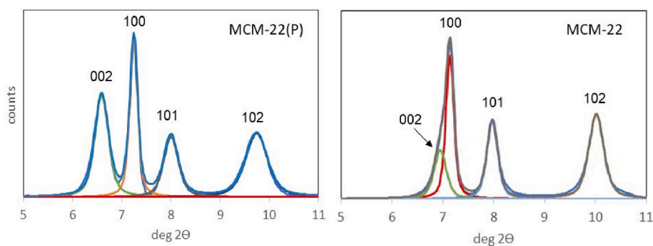
Fig. 2. Evolution of the XRD pattern of MCM-22(P) upon calcination, with decrease of the c cell parameter and formation of MCM-22.
