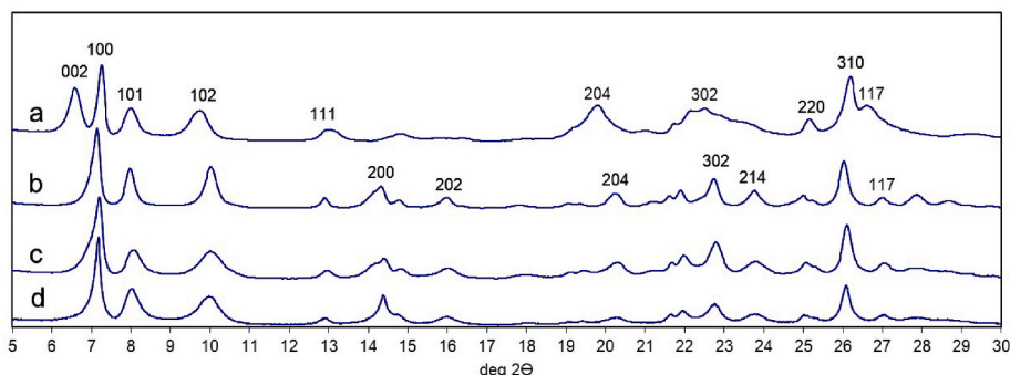
Fig. 8. Evolution of the XRD pattern of MWW(P) upon calcination or treatment by concentrated \text{HNO}_3 : samples MWW(P) (a), MWW(P)C (b), AA (c), AAC (d).
