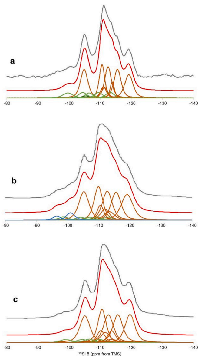
Fig. 9. ^{29}\text{Si} MAS-NMR spectra of samples MWW(P)C (a), AA (b) and AAC (c). For each sample, the top trace is the experimental spectrum, the mid trace is the simulated one, and the lower traces are the components of the deconvolution.
