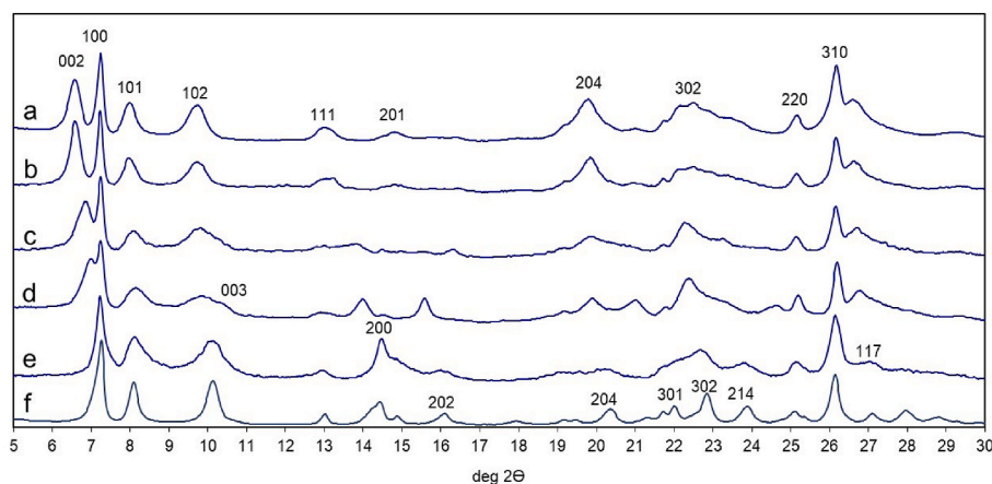
Fig. 6. Evolution of the XRD pattern of MWW(P) upon treatment by diluted \text{HNO}_3 in organic solvent in the presence of \text{Cu}^{2+} cations: samples MWW(P) (a), CupH4E-4 (b), CupH4E-3 (c), CupH4E-2 (d), CupH4E-2C (e), MWW(P)C (f).
