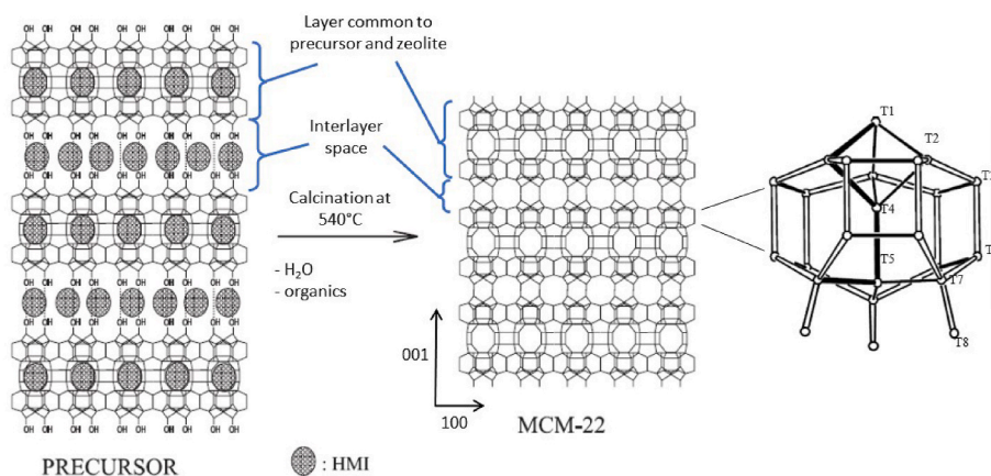
Fig. 1. Condensation of the layers of MCM-22(P) to form MCM-22 and nomenclature of the tetrahedra of the MWW structure. HMI is hexamethyleneimine. Modified from Pergher et al. [34] and from the IZA structure database [35].
