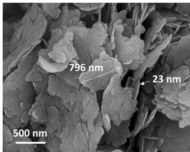
Fig. 4. Scanning electron micrograph of MWW(P)C sample.
