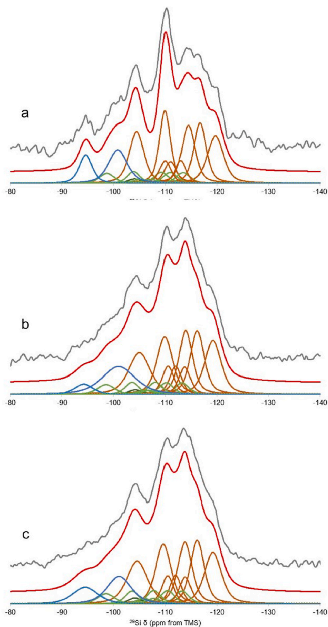
Fig. 5. ^{29}\text{Si} MAS-NMR spectra of samples MWW(P) (a), Ph1 (b) and CupH4E-2 (c). For each sample, the top trace is the experimental spectrum, the mid trace is the simulated one, and the lower traces are the components of the deconvolution.
