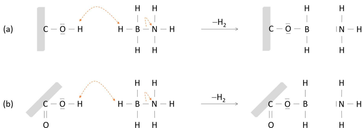
Figure 8. Interactions and reactions between (a) surface \text{CO}-\text{H} and \text{AB} , and (b) surface \text{COO}-\text{H} and \text{AB} , resulting in the formation of surface \text{CO}-\text{B} and \text{COO}-\text{B} bonds, the release of \text{H}_2 and the generation of \text{NH}_3 .
