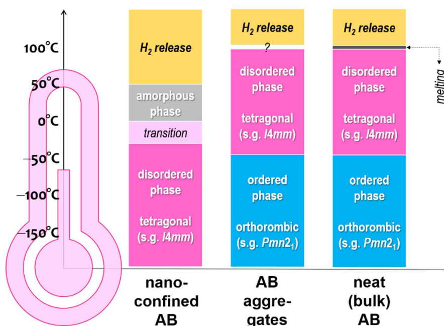
Figure 7. Phase transformation of confined AB, aggregates of AB (i.e. outside the porosity of the scaffold), and bulk AB, from -193 to 150\text{ }^{\circ}\text{C} .
