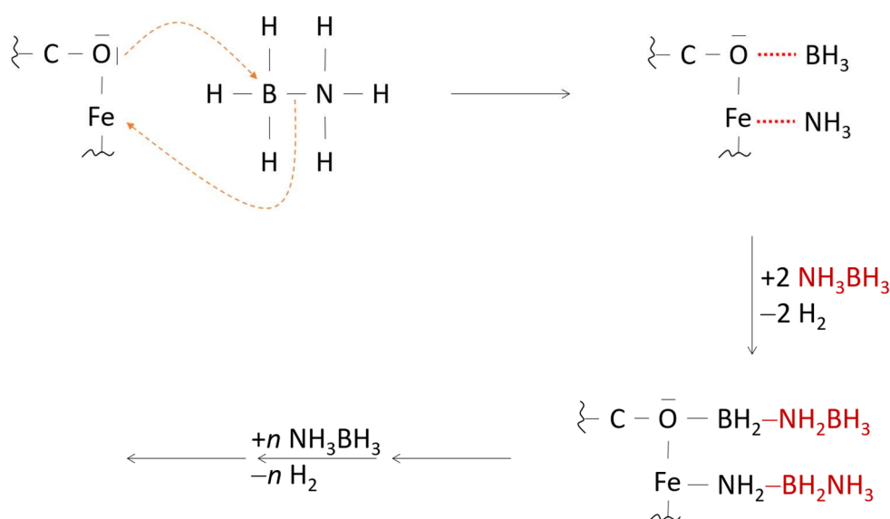
Figure 10. Interaction of AB with the Fe-MIL-53 pore surface, via \text{O}\cdots\text{BH}_3 and \text{Fe}\cdots\text{NH}_3 , resulting in \text{CO}-\text{BH}_2 and \text{Fe}-\text{NH}_2 groups upon reaction with 2 AB molecules.
