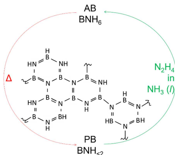
Figure 3. Hydrogen cycle with AB and PB ( \text{BNH}_{<2} ): dehydrogenation of AB under heating resulting in PB, and chemical recycling of PB into AB in the presence of \text{N}_2\text{H}_4 in liquid \text{NH}_3 .
