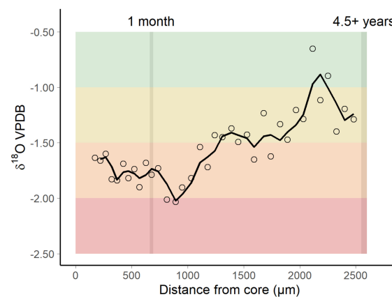
Figure 4. Measurements of \delta^{18}\text{O} values made by SIMS across the otolith growth axis from core to the near-edge in an adult yellowfin tuna. The 134 cm FL individual was captured in South Africa in May 2018. Dots are values measured at each spot, and solid line represents the mobile mean. The approximate location of the first month of life and 4.5+ years are indicated.
