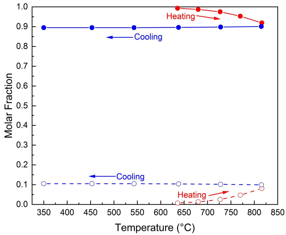
Figure 8. Variation of molar fraction of USiO 4 (solid circles) and UO 2 (open circles) upon heating (red) and then cooling (blue).
