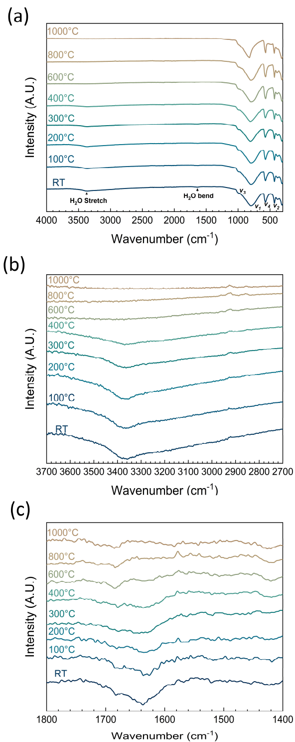
Figure 10. FTIR performed on pristine and calcinated stetindite for temperatures ranging from room temperature to 1000°C in the regions (a) 4000-300 \text{cm}^{-1} , (b) 3700-2700 \text{cm}^{-1} and (c) 1800-1400 \text{cm}^{-1} . Arrows and labels indicate what the various vibrational bands are attributed. \nu_1 , \nu_2 , \nu_3 , \nu_4 are the 4 normal internal modes of vibration.
