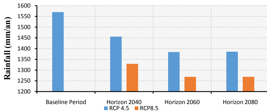
Figure 10. Evolution of annual rainfall compared to the baseline period (1960-1981).
