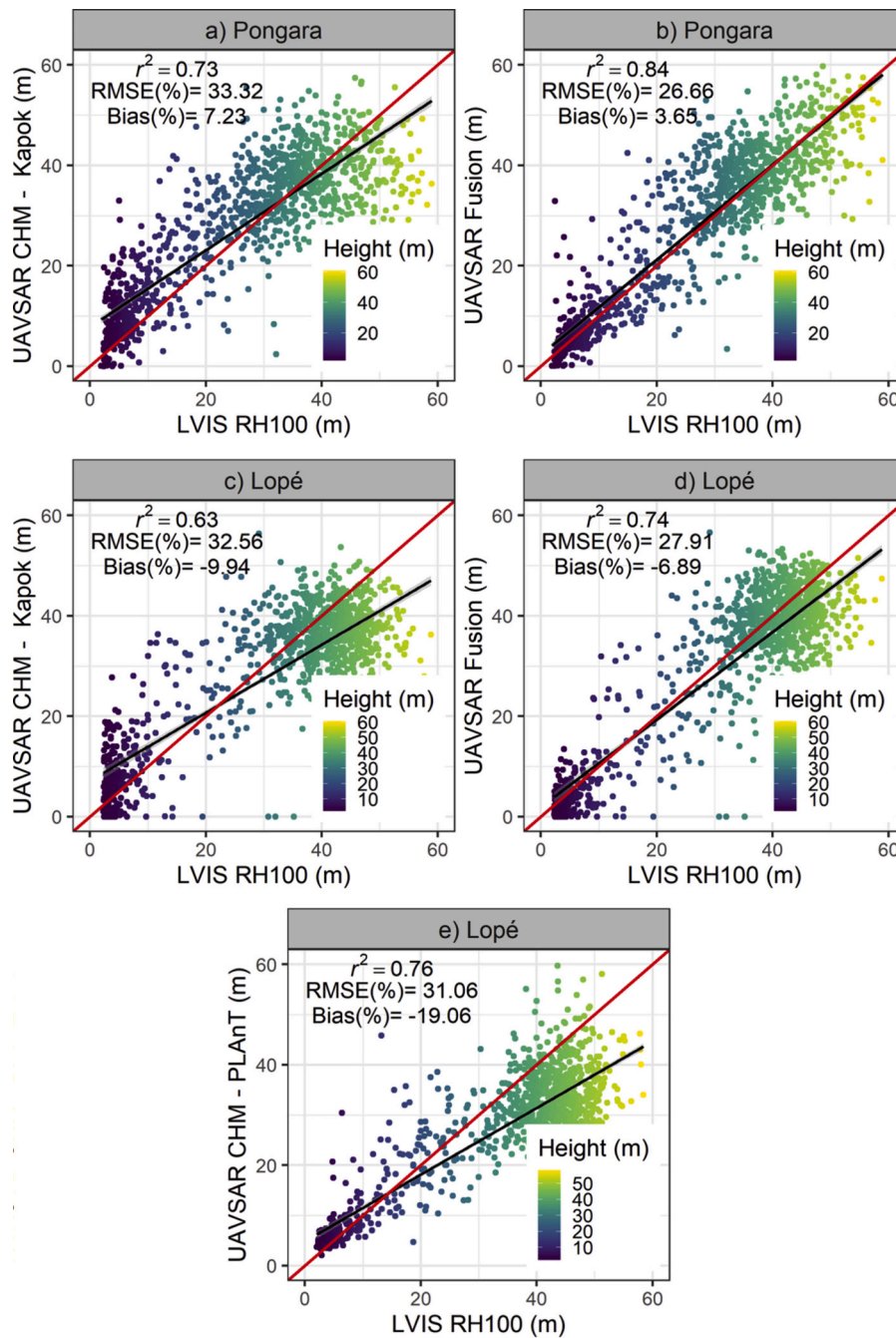
Fig. 5. Comparison of LVIS Rh 100 standard height products with 3 UAVSAR Pol-InSAR height products CHM Kapok (Denbina et al, 2018), CHM Fusion (Denbina et al, 2018) and CHM Plant (Lavalle et al., 2018).
