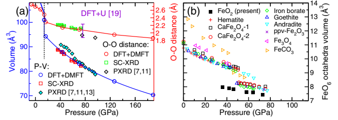
FIG. 1. Compressional behavior of HP-PdF 2 -type \text{FeO}_2 : (a) lattice volume and O–O distance obtained by DFT + DMFT at T = 1160 K in comparison to XRD data. DFT + DMFT predicts a spin-state transition at \sim 14 GPa, depicted by a dashed vertical line. (b) Pressure dependence of volumes of the \text{FeO}_6 octahedra in various compounds according to Ref. [46].
