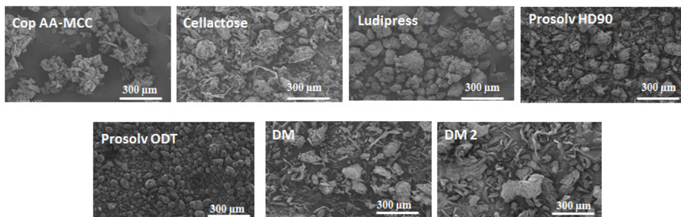
Figure 1. SEM images of the different co-processed excipients (Cop AA-MCC, Cellactose, Ludipress, Prosohv HD90, and Prosohv ODT) and the dry mixtures (DM and DM2).
