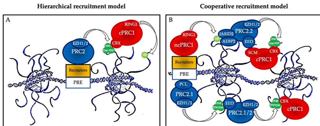
Figure 2. Polycomb group protein chromatin recruitment models. (A) Hierarchical recruitment model: PRC2 is recruited first and deposits H3K27me 3 on chromatin via its catalytical subunit EZH1 or EZH2; then, canonical PRC1 (cPRC1) is recruited by a chromobox member CBX on the H3K27me 3 mark and deposits H2AK119ub 1 on chromatin via its catalytical subunit RING1. (B) Cooperative recruitment model: ncPRC1 complexes deposit H2AK119ub, which recruits PRC2.2 via its JARID2 and AEBP2 subunits. In parallel, PRC2.1 is recruited to unmethylated CpG island DNA via its PCL subunits. PRC2.1 and PRC2.2 complexes deposit H3K27me 3 , and this mark recruits both more copies of PRC2 and cPRC1. Mutual interactions between the core PRC2 member EED and the cPRC1 member SCM further stabilize their recruitment. PRE: polycomb responsive element (considered as CpG islands in mammals).
