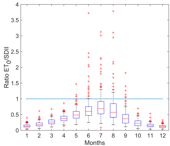
Figure 4. Box plot of the monthly ratios between ET_0 and SDII. On each box, the central mark is the median, the edges of the box are the 25th and 75th percentiles, and the whiskers extend to \pm 1.5 interquartile range.
