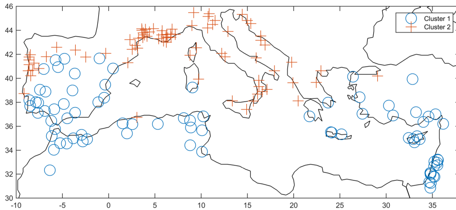
Figure 6. Clustering result of monthly net precipitation ( P - ET_0 ).
