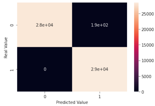
Figure 7: CNN Confusion Matrix
