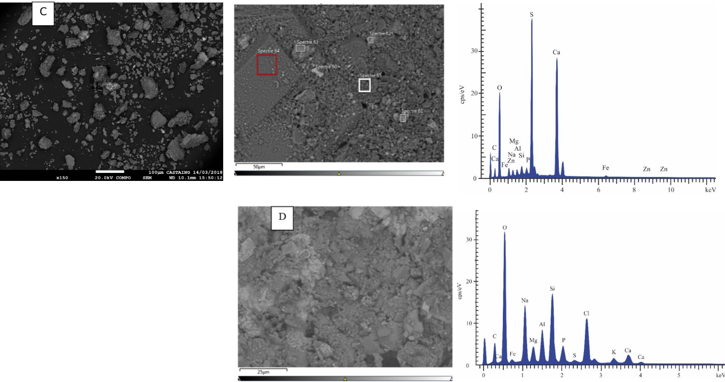
Figure SI-1. Morphology of atmospheric deposition and associated chemical spectra, analysed by SEM-EDX: A) Mining area and day mineral spectra (ex: K adinite); B) Mining area and lead sulphate spectra (ex: M gnesite); C) Urban area and calcium sulphate (ex: G ypsum); D) Coastal zone and halite spectra.
