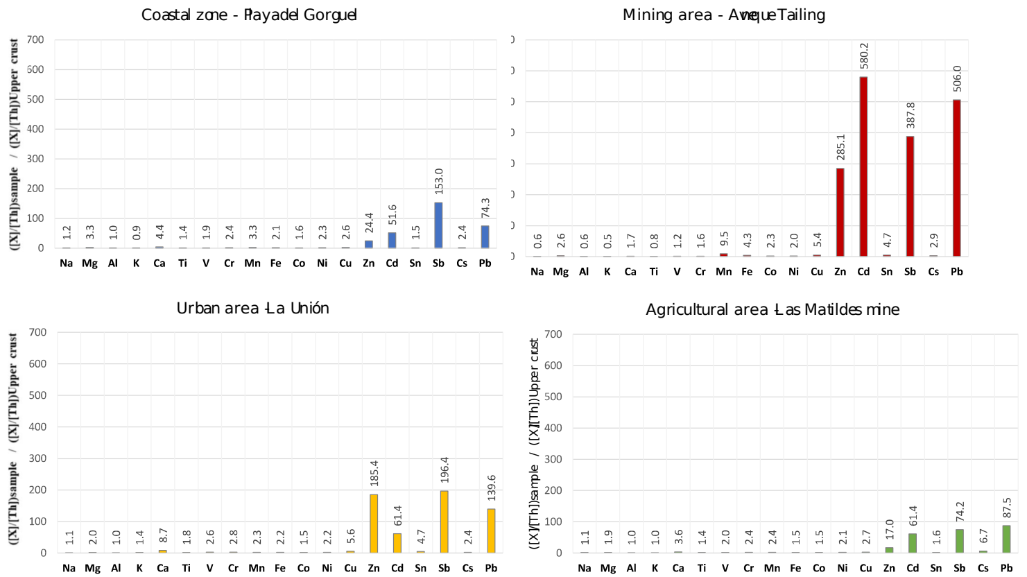
Figure 3. Enrichment factors (EF) of atmospheric dusts relative to the upper Earth's crust. The same scale is used to better assess variation between sites.
