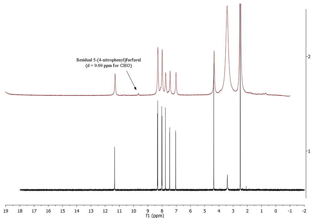
Figure 6. Assessment of dantrolene identity by comparison of ^1\text{H} NMR spectra for LAG reaction (red spectrum) vs. the analytical sample prepared by planetary ball mill 51 (black spectrum).
