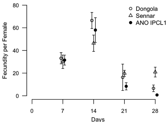
Fig. 2. Fecundity (mean \pm SEM) per female for the four generational cycles, for the three strains of An. arabiensis .
