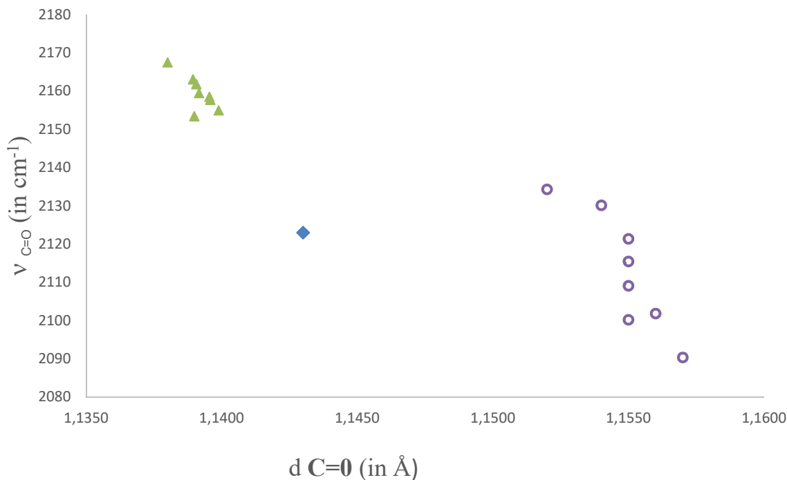
Figure 3. CO in faujasite Y exchanged with \text{Na}^{\text{I}} or \text{Cu}^{\text{I}} : \nu_{C=O} stretching frequency (in \text{cm}^{-1} ) as a function of the C=O distance (in \text{\AA} ) calculated with PBE/PAW method in (\text{CO})_8\text{Na}_8\text{Al}_{14}\text{O}_{98}\text{Si}_{34} (triangles), (\text{CO})_8\text{Cu}_8\text{Al}_{14}\text{O}_{98}\text{Si}_{34} (circles) and \text{CO}_{\text{gas}} (diamond, modeled in a periodic box).
