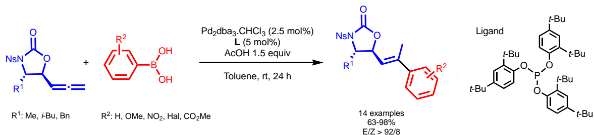
Scheme 55: Pd(0)-catalyzed hydroarylation of allenylloxazolidinones with arylboronic acids.
