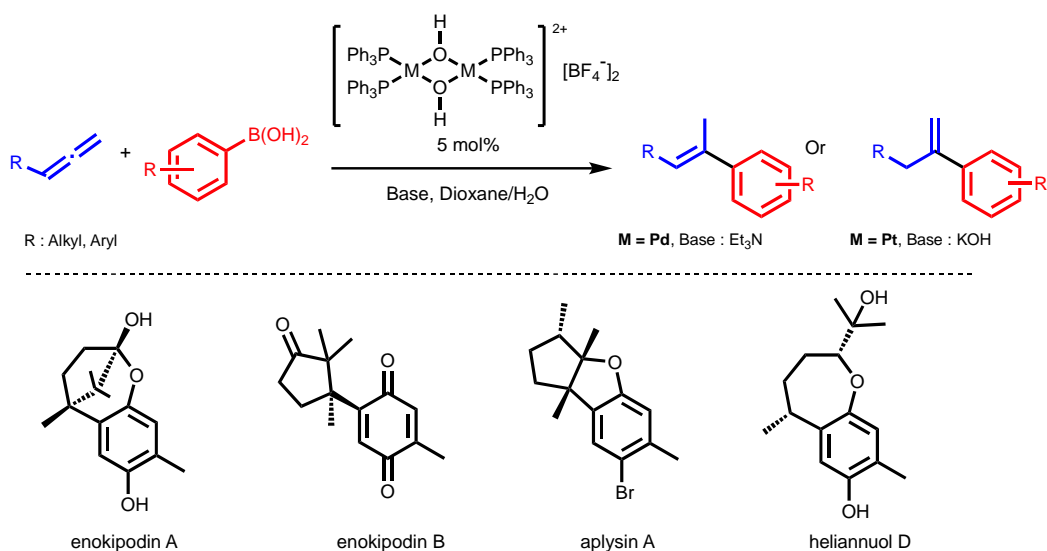
Scheme 54: Hydroarylation of allenenes with aryl boronic acids by Pt- and Pd-catalysis assistance.
