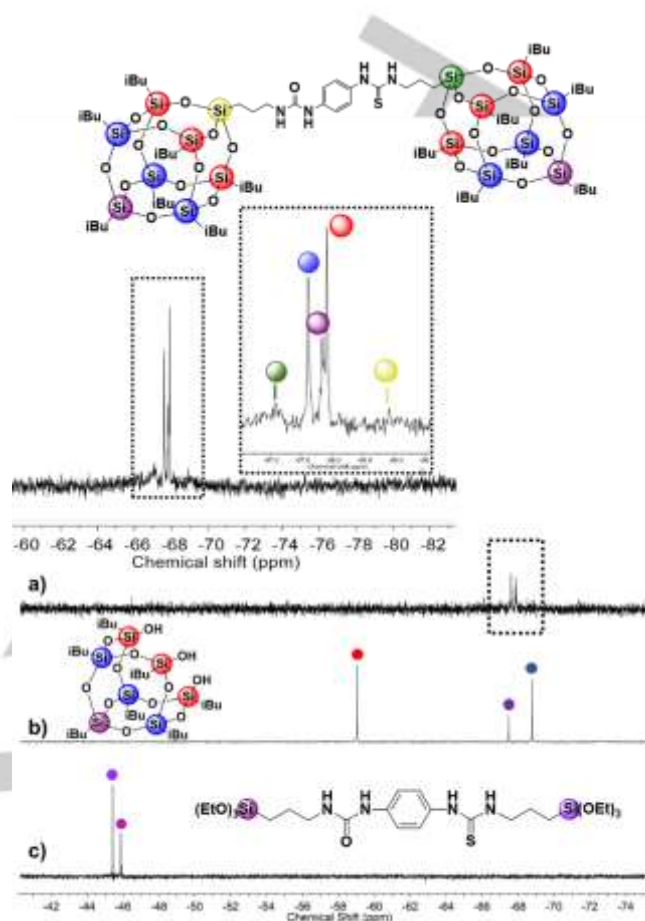
Figure 6. ^{29}\text{Si} solution NMR spectra of a) urea-thiourea dumbbell, 9 , b) partially condensed T 7 -triol and c) urea-thiourea bistriethoxysilyl linker, 5
