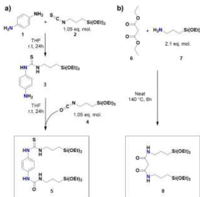
Scheme 2. a) Synthesis of urea-thiourea linker, 5 . b) Synthesis of malonamide linker, 8 .
