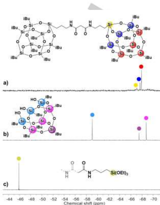
Figure 8. 29 Si solution NMR spectra of a) malonamide dumbbell, 10 , b) partially condensed T 7 -triol and c) malonamide linker, 8
