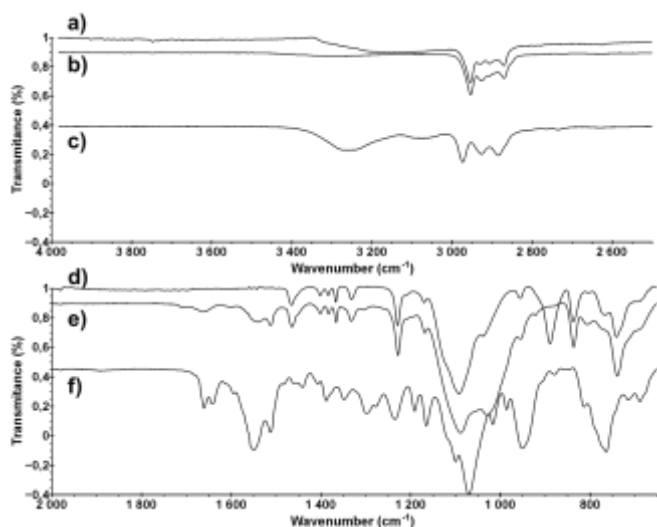
Figure 7. FT-IR spectra (4000-2000 cm -1 ) of a) Partially condensed T 7 -triol, b) Urea-thiourea dumbbell, 9 , and c) Urea-thiourea linker, 5 . FT-IR spectra (2000-600 cm -1 ) of d) Partially condensed T 7 -triol, e) Urea-thiourea dumbbell, 9 , and f) Urea-thiourea linker, 5 .
