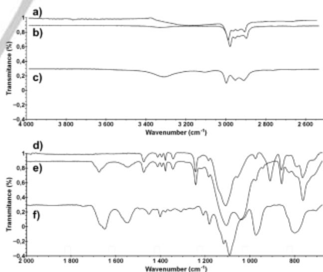
Figure 9. FT-IR spectra (4000-2500 cm -1 ) of a) Partially condensed T 7 -triol, b) Malonamide dumbbell, 10 and c) Malonamide bistrithoxysilane linker, 8 . FT-IR spectra (2000-600 cm -1 ) of d) Partially condensed T 7 -triol, e) Malonamide dumbbell, 10 and f) Malonamide bistrithoxysilane linker, 8 .
