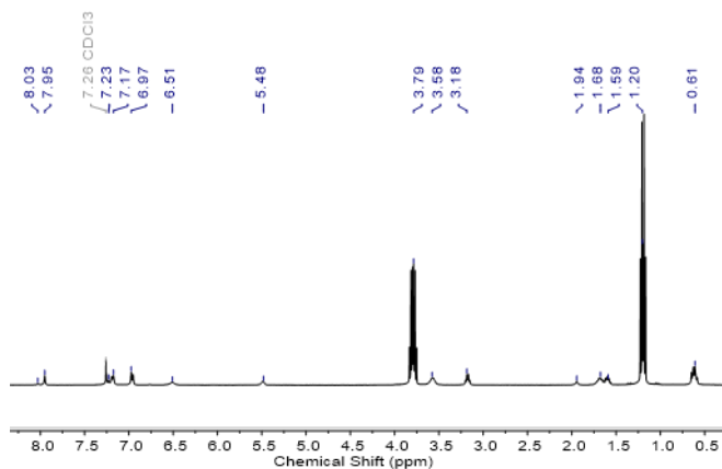
Figure 2. ^1\text{H} NMR spectrum of the urea-thiourea bistrithoxysilane linker 5 in \text{CDCl}_3 .
