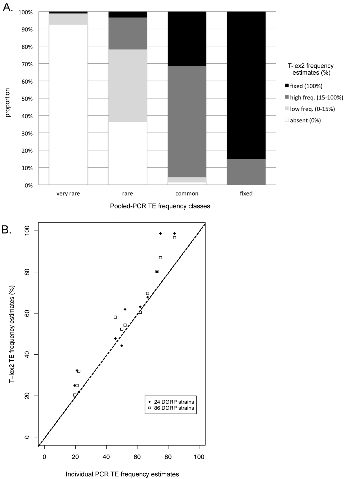
Figure 5. TE frequency estimates using D. melanogaster single strains. (A) Comparison of the frequency estimates of 709 TE insertions using T-lex2 and pooled PCR approach. (B) Frequency estimates of 11 TE insertions using T-lex2 and single PCR approach.
