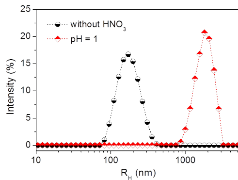
Figure 3: Dynamic light scattering measurements at \theta = \text{CP} + 10 \text{ }^\circ\text{C} for P(CPAAm6C) 5 \text{ g}\cdot\text{L}^{-1} without nitric acid ( \theta = 52 \text{ }^\circ\text{C} ) and at pH = 1 ( \theta = 42 \text{ }^\circ\text{C} ).
