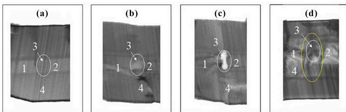
Figure 8. X-ray topography of cross sections of \text{GaPO}_4 crystals grown on c\{0001\} seed plates (thickness is near to 1.5 mm) included some defects: (a) twin, (b) dislocation, (c) crack and (d) all together. 1, 2—initial seed plates; 3—defect (twin, dislocation or crack), 4—overgrown layer.
