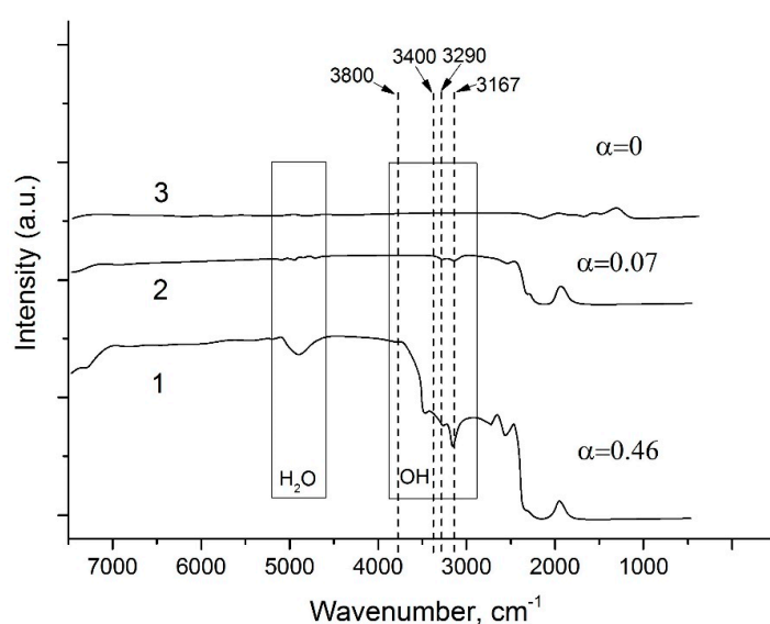
Figure 9. IR spectra of \text{GaPO}_4 crystals obtained under follow conditions: 1—hydrothermal solution, 9 M \text{H}_3\text{PO}_4 /12 M \text{HCl} (80/20), T = 240 ^\circ\text{C} , dT = 10 ^\circ\text{C} , refluxing method, isometric crystals; 2—hydrothermal solution, 6 M \text{H}_2\text{SO}_4 , T = 230 ^\circ\text{C} , dT = 4 ^\circ\text{C} , temperature gradient method, plate-like crystals, 3—flux, lithium molybdate, T = 750 – 900 ^\circ\text{C} , decreasing of temperature, millimeter size crystals.
