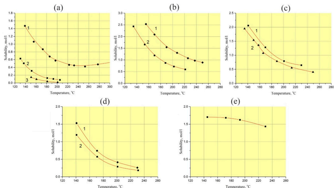
Figure 1. Solubility of \text{GaPO}_4 in aqueous solutions (at pressure of 5–20 bar): (a) \text{H}_3\text{PO}_4 , 1–15 M, 2–7.5 M, 3–5 M; (b) \text{H}_2\text{SO}_4 , 1–9 M, 2–6.5 M; (c) 15 M \text{H}_3\text{PO}_4 /9 M \text{H}_2\text{SO}_4 in vol. proportions (%): 1–20/80, 2–50/50; (d) 9 M \text{H}_3\text{PO}_4 /6 M \text{H}_2\text{SO}_4 in vol. proportions (%): 1–20/80, 2–70/30; (e) 6 M \text{HCl} [30].
