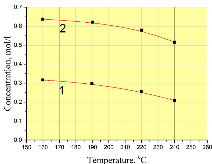
Figure 2. \text{GaPO}_4 concentration in 9\text{ M H}_3\text{PO}_4/6\text{ M HCl} (vol. proportion 95/5%) at temperature 160\text{--}240^\circ\text{C} and pressure 5–20 bar. 1—with crystallization; 2—without crystallization.
