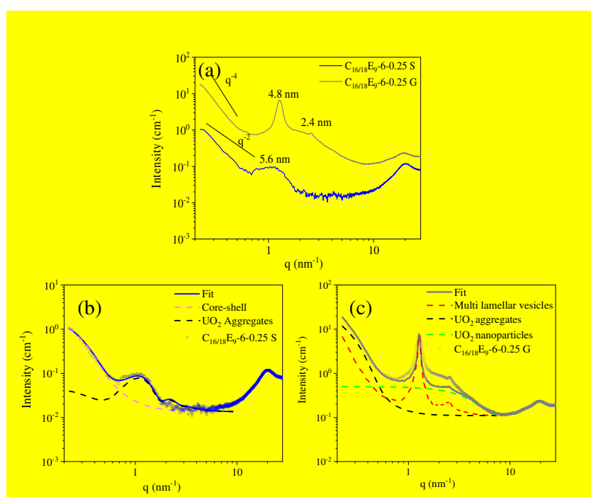
Figure 5. (a) SWAXS patterns of the supernatants C_{16/18}E_9-6-0.25 S and the dense gel C_{16/18}E_9-6-0.25 G of the sample C_{16/18}E_9-6-0.25 ; (b) Experimental and simulated SWAXS patterns of C_{16/18}E_9-6-0.25 S; (c) Experimental and simulated SWAXS patterns of C_{16/18}E_9-6-0.25 G.
